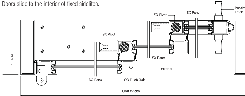
Horizontal Section
